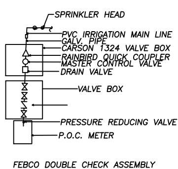
SCHEMATIC OF POINT OF CONNECTION NTS
