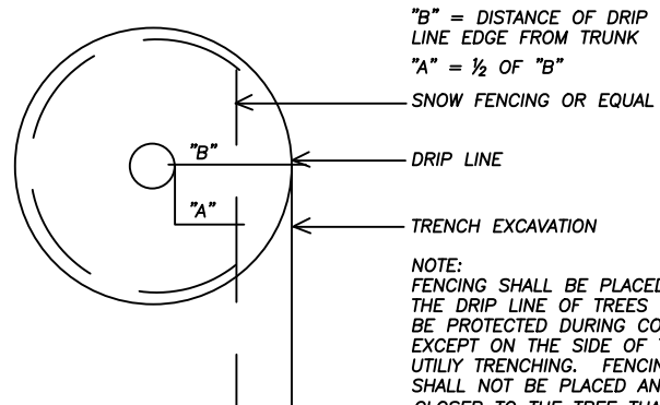
TEMPORARY TREE PROTECTION PLAN
