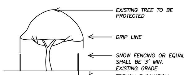
TREE PROTECTION DETAIL NTS
